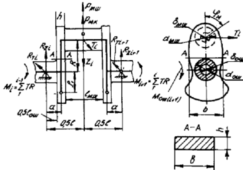
Computational scheme of full-supporting crankshaft
