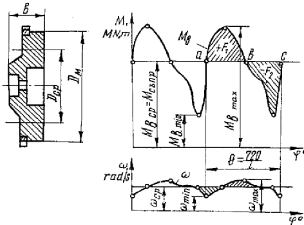
Fluctuation of the torque and angular velocity
